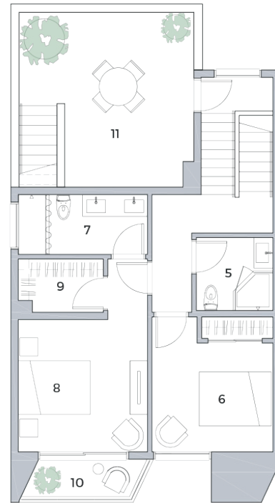
LEVEL 2 AND ROOF LEVEL
